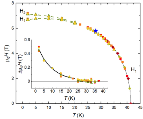
\text{UIrSi}_3 phase diagram complimented with acoustic data[2] (grey color existing diagram [1]).
